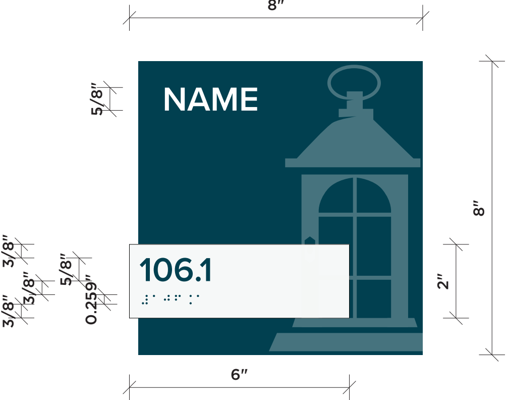
UNIT ID SIGN
