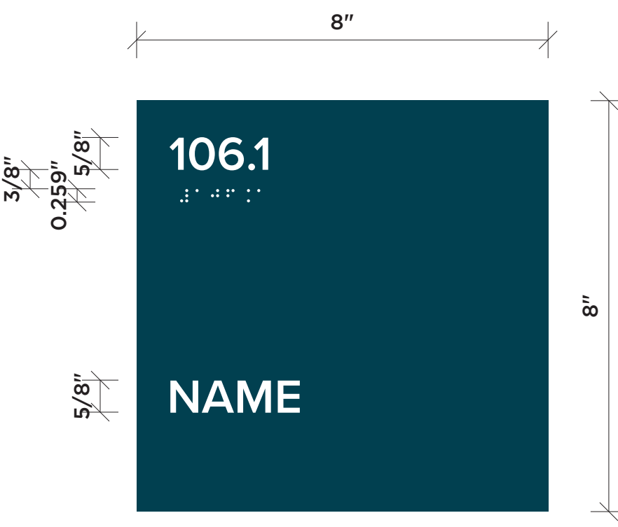
UNIT ID SIGN
