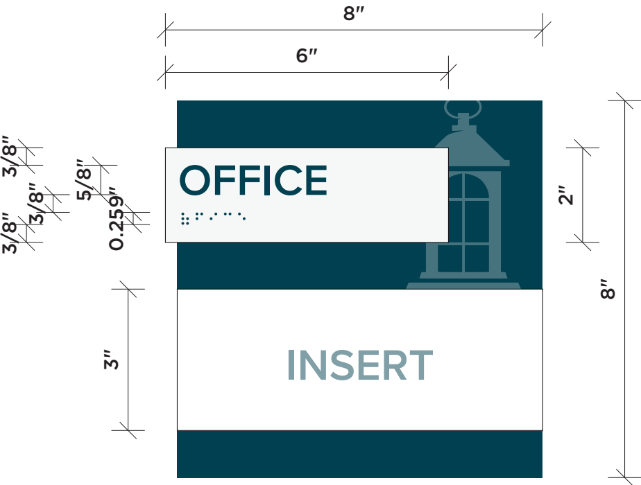
OFFICE WITH INSERT SIGN
