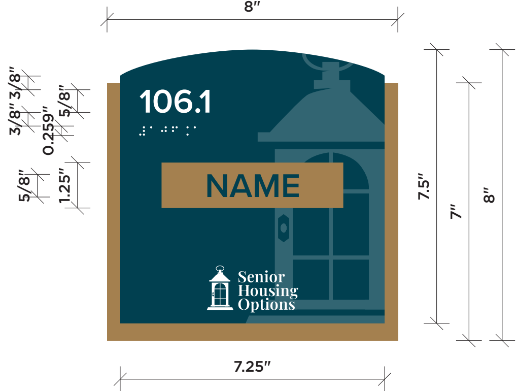
UNIT ID SIGN
