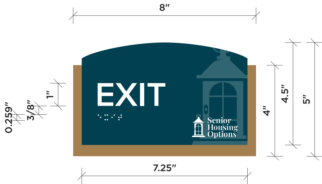
EXIT AND LEVEL ID SIGN
