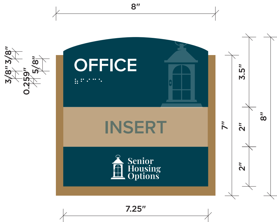
OFFICE WITH INSERT SIGN
