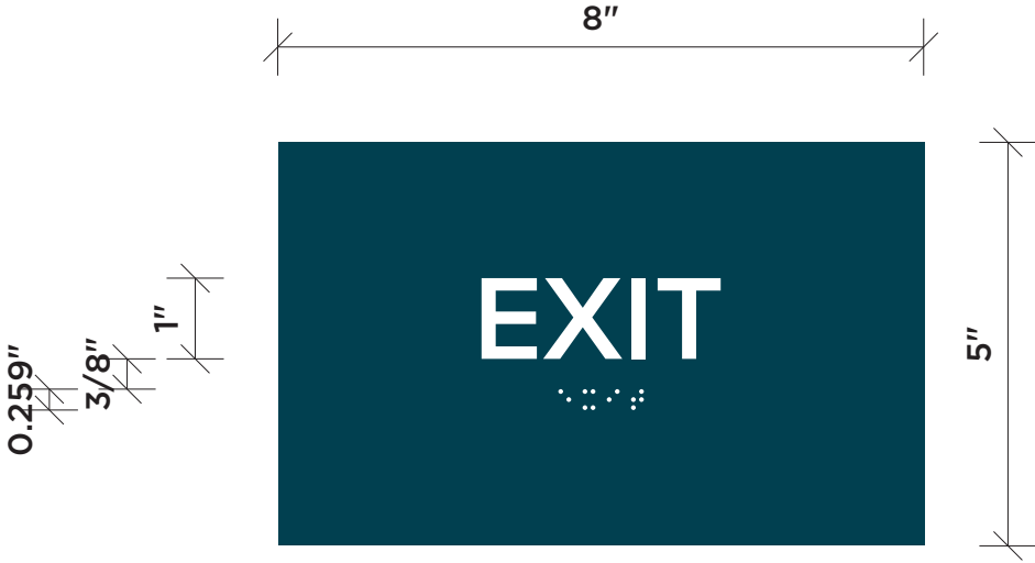
EXIT AND LEVEL ID SIGN
